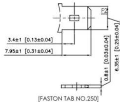
Detail A Drawing(3:1)
