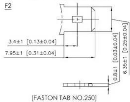
Detail A Drawing(3:1)
